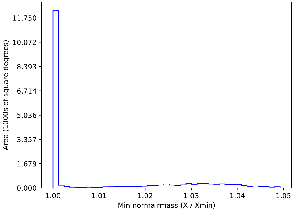
ddf_acor_sf20_lsf0_lsr0_v3.4_10yrs WFD g band: Min normairmass
