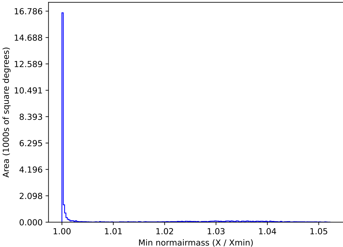
ddf_acor_sf20_lsf0_lsr0_v3.4_10yrs All sky g band: Min normairmass
