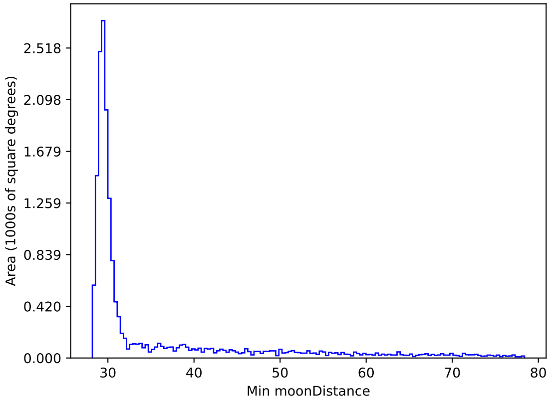
ddf_acor_sf20_lsf0_lsr0_v3.4_10yrs WFD y band: Min moonDistance
