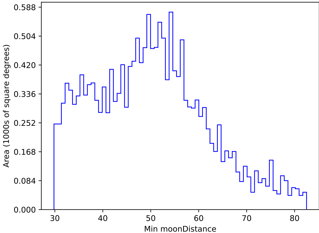
ddf_acor_sf20_ls0_lsr0_v3.4_10yrs WFD u band: Min moonDistance
