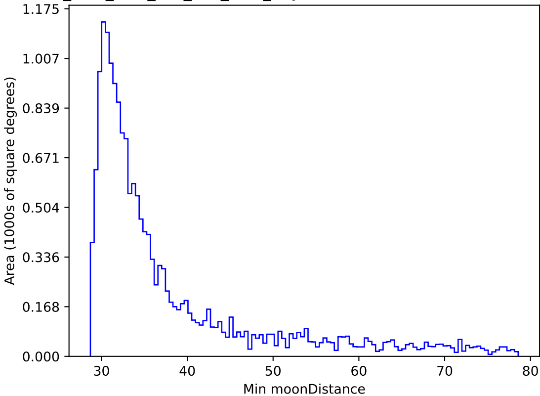
ddf_acor_sf20_lsf0_lsr0_v3.4_10yrs WFD r band: Min moonDistance
