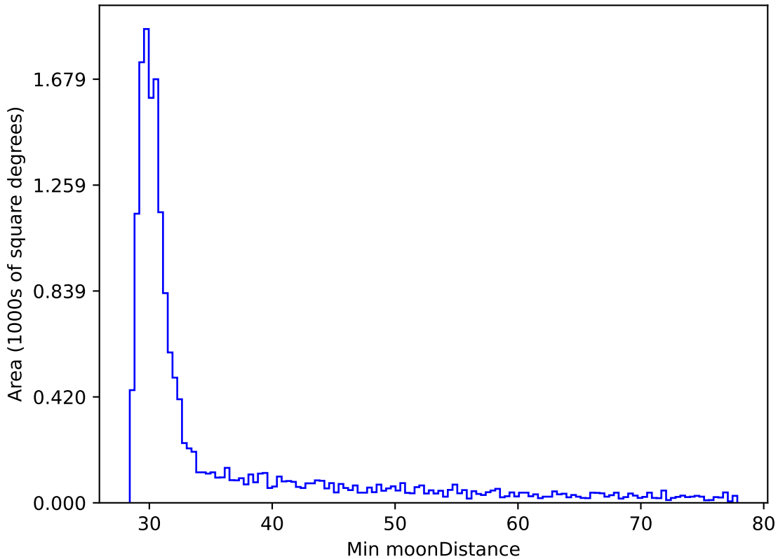
ddf_acor_sf20_lsf0_lsr0_v3.4_10yrs WFD i band: Min moonDistance
