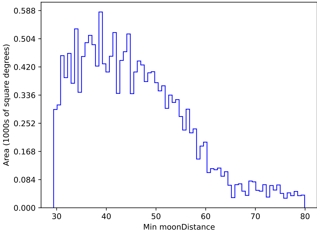
ddf_acor_sf20_ls0_lsr0_v3.4_10yrs WFD g band: Min moonDistance
