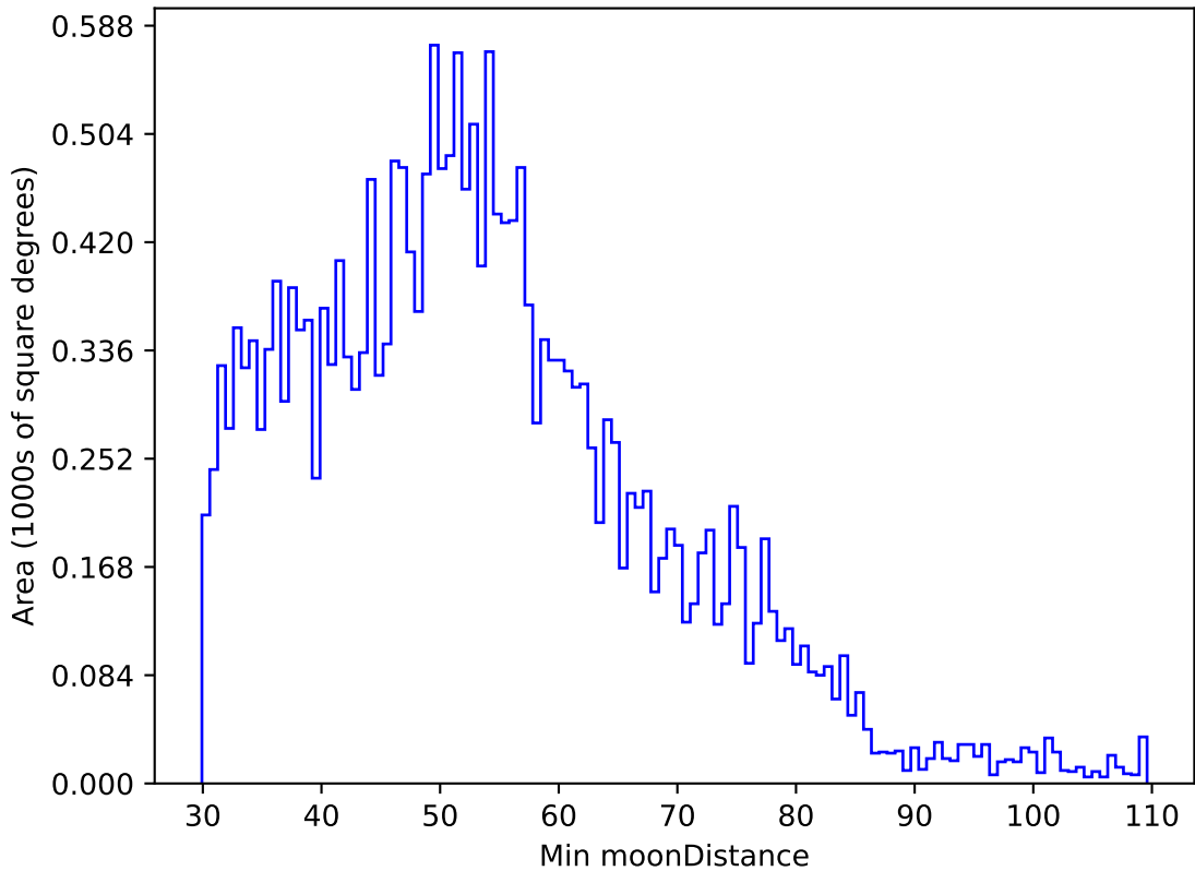
ddf_acor_sf20_lsf0_lsr0_v3.4_10yrs All sky u band: Min moonDistance
