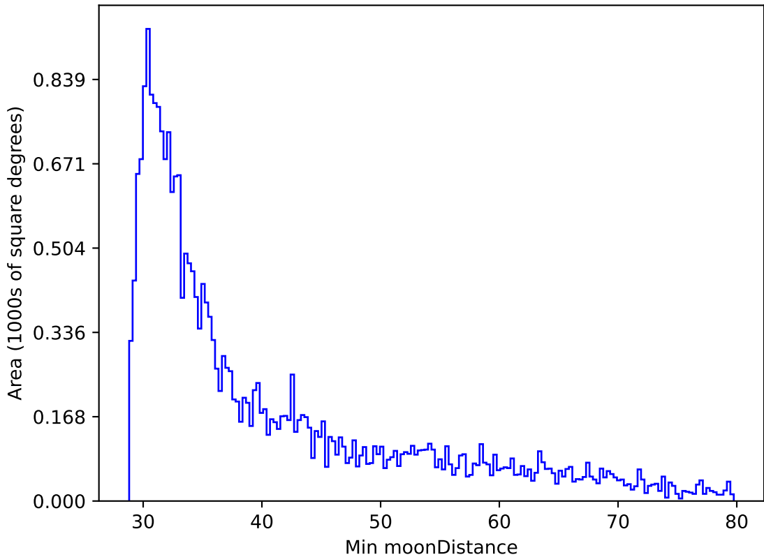
ddf_acor_sf20_lsf0_lsr0_v3.4_10yrs All sky r band: Min moonDistance
