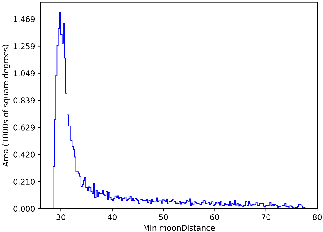
ddf_acor_sf20_lsf0_lsr0_v3.4_10yrs All sky i band: Min moonDistance
