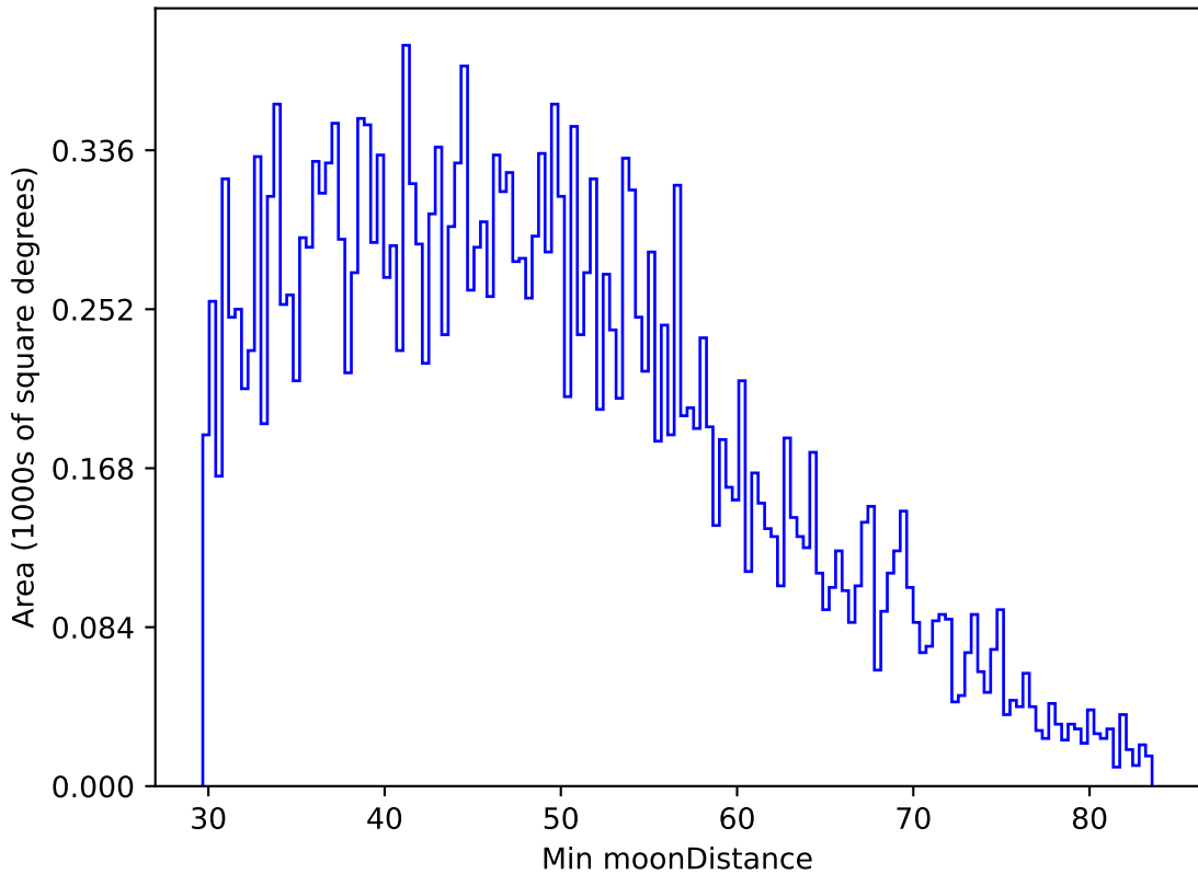
ddf_acor_sf20_lsf0_lsr0_v3.4_10yrs All sky g band: Min moonDistance
