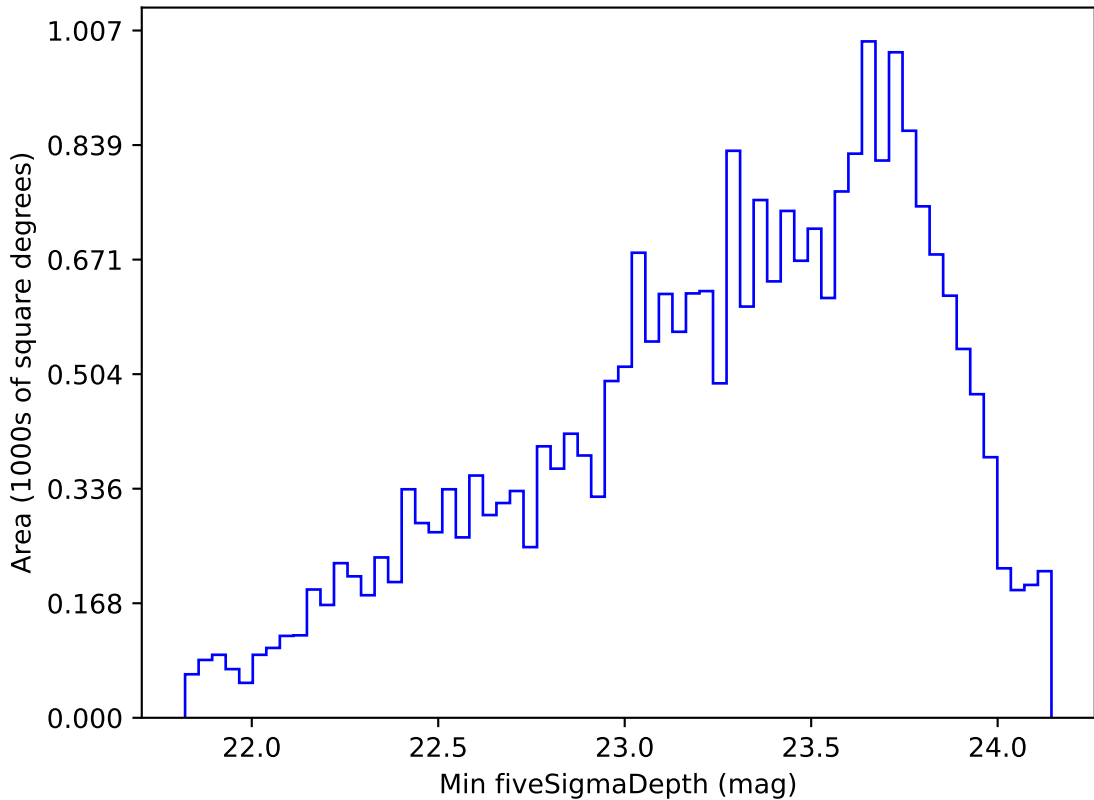
ddf_acor_sf20_lsf0_lsr0_v3.4_10yrs Yr 1 r band: Min fiveSigmaDepth
