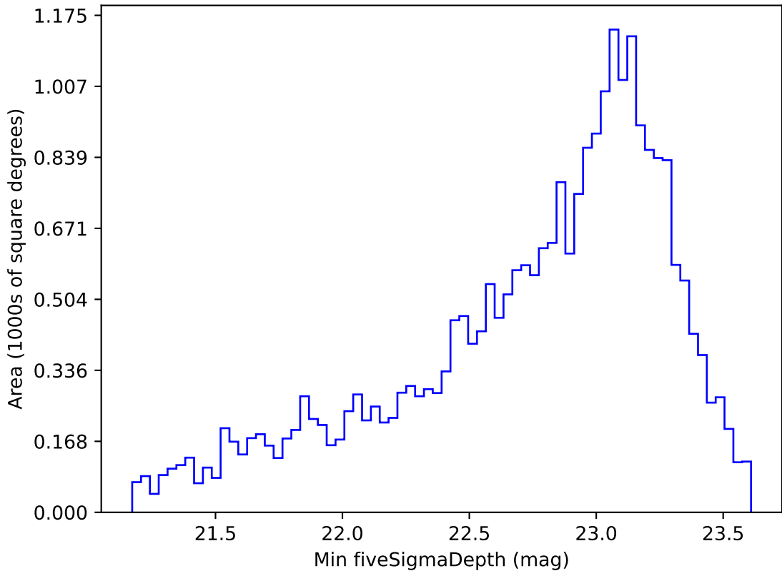
ddf_acor_sf20_lsf0_lsr0_v3.4_10yrs Yr 1 i band: Min fiveSigmaDepth
