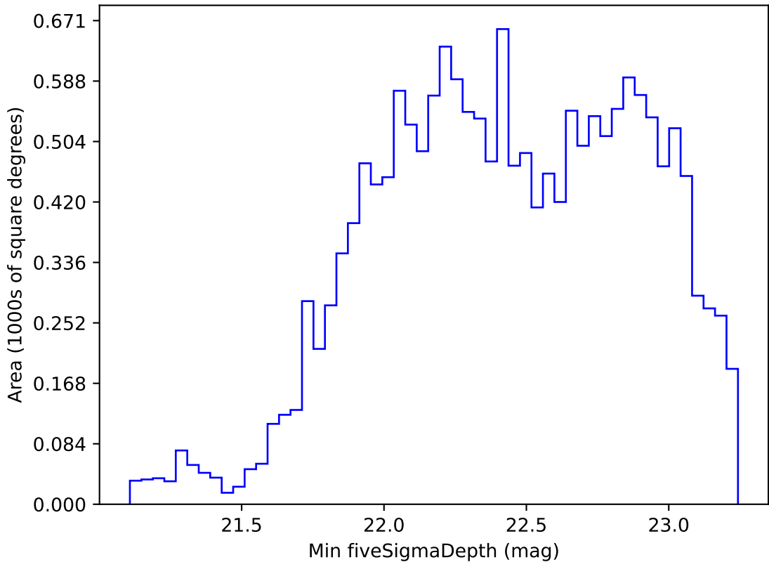
ddf_acor_sf20_lsf0_lsr0_v3.4_10yrs WFD r band: Min fiveSigmaDepth
