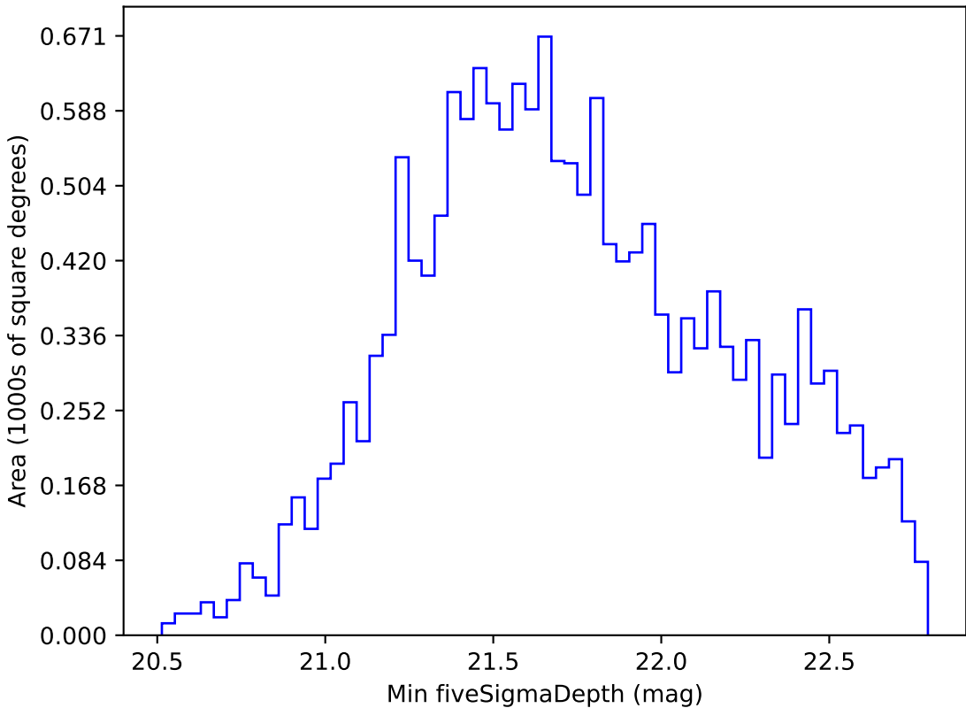
ddf_acor_sf20_lsf0_lsr0_v3.4_10yrs WFD i band: Min fiveSigmaDepth
