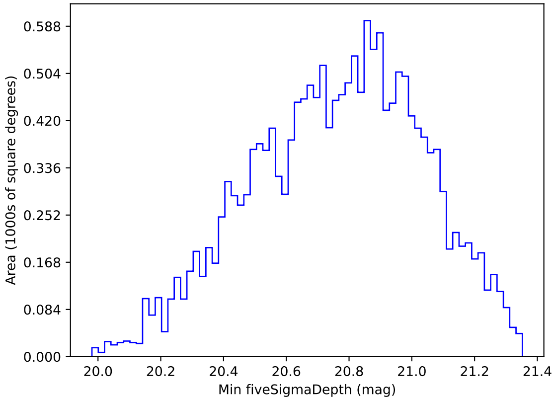
ddf_acor_sf20_lsf0_lsr0_v3.4_10yrs WFD all bands: Min fiveSigmaDepth
