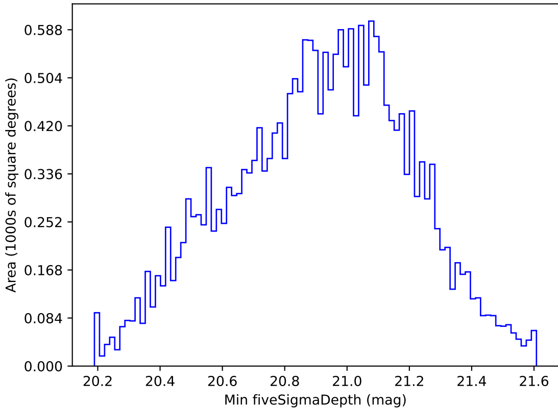
ddf_acor_sf20_lsf0_lsr0_v3.4_10yrs All sky y band: Min fiveSigmaDepth
