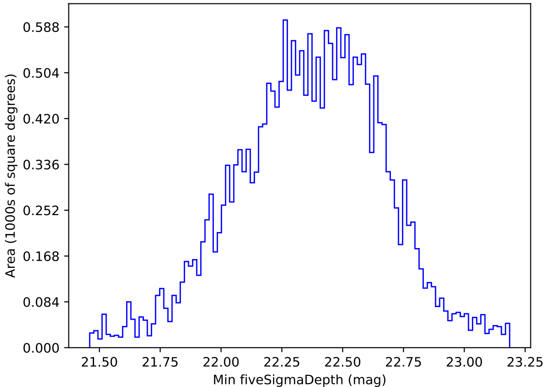
ddf_acor_sf20_ls0_lsr0_v3.4_10yrs All sky u band: Min fiveSigmaDepth
