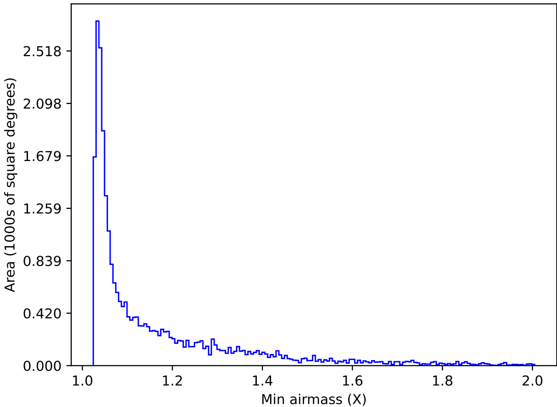
ddf_acor_sf20_lsf0_lsr0_v3.4_10yrs Yr 1 r band: Min airmass
