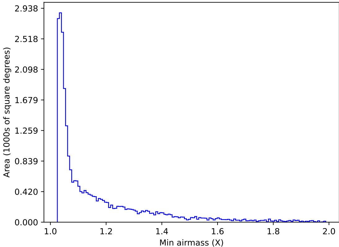
ddf_acor_sf20_lsf0_lsr0_v3.4_10yrs Yr 1 i band: Min airmass
