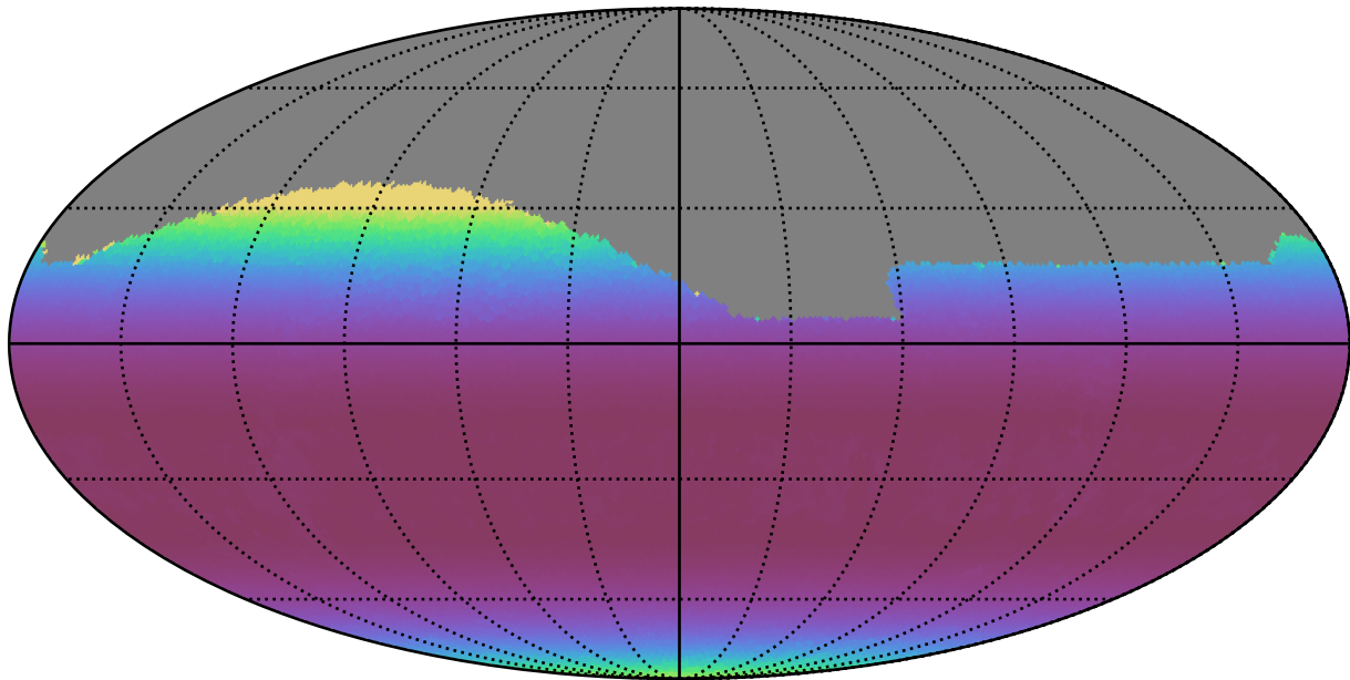
ddf_acor_sf20_lsf0_lsr0_v3.4_10yrs Yr 1 all bands: Min airmass
