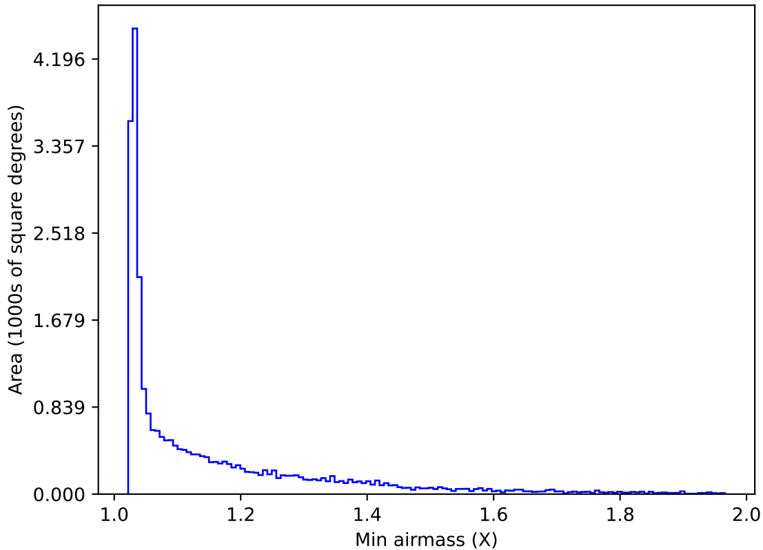
ddf_acor_sf20_lsf0_lsr0_v3.4_10yrs Yr 1 all bands: Min airmass
