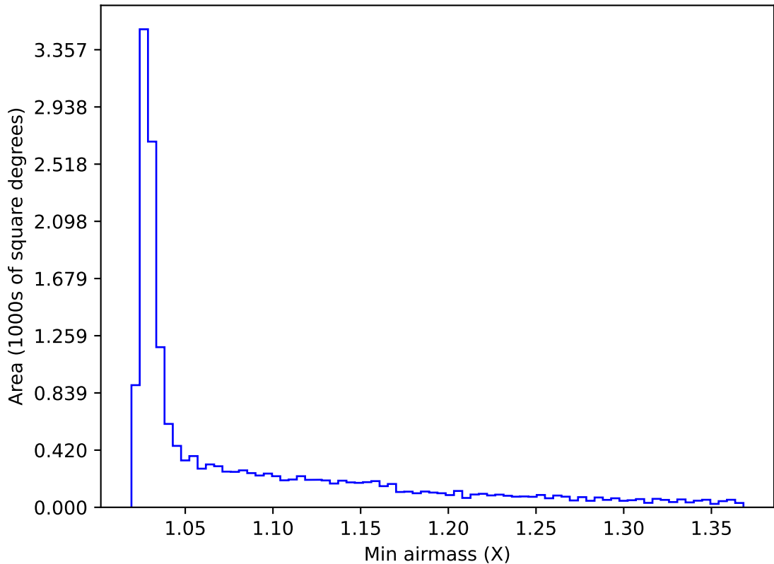
ddf_acor_sf20_lsf0_lsr0_v3.4_10yrs WFD z band: Min airmass
