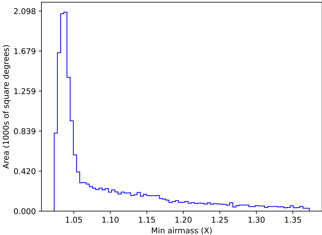
ddf_acor_sf20_lsf0_lsr0_v3.4_10yrs WFD g band: Min airmass
