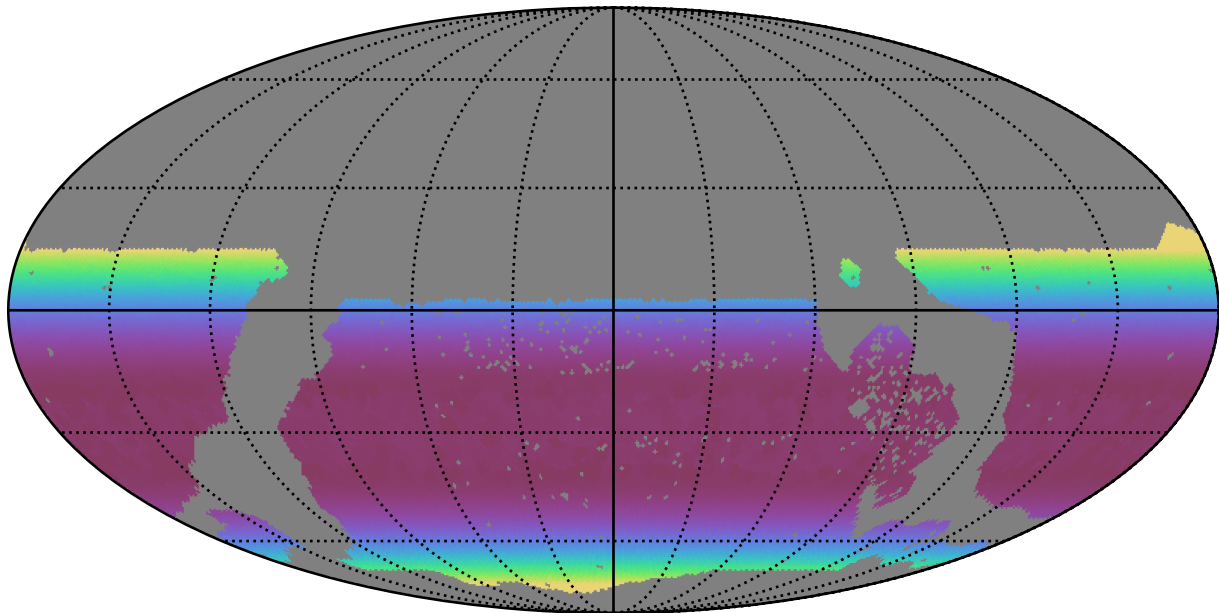
ddf_acor_sf20_lsf0_lsr0_v3.4_10yrs WFD all bands: Min airmass
