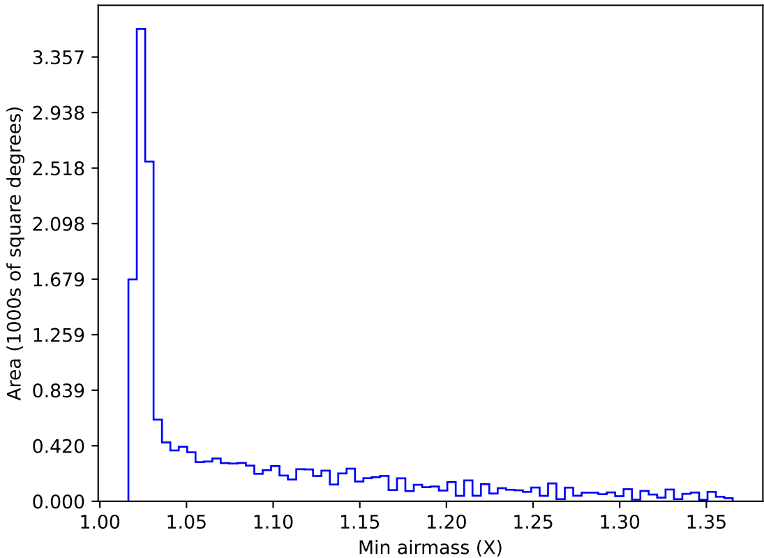
ddf_acor_sf20_lsf0_lsr0_v3.4_10yrs WFD all bands: Min airmass
