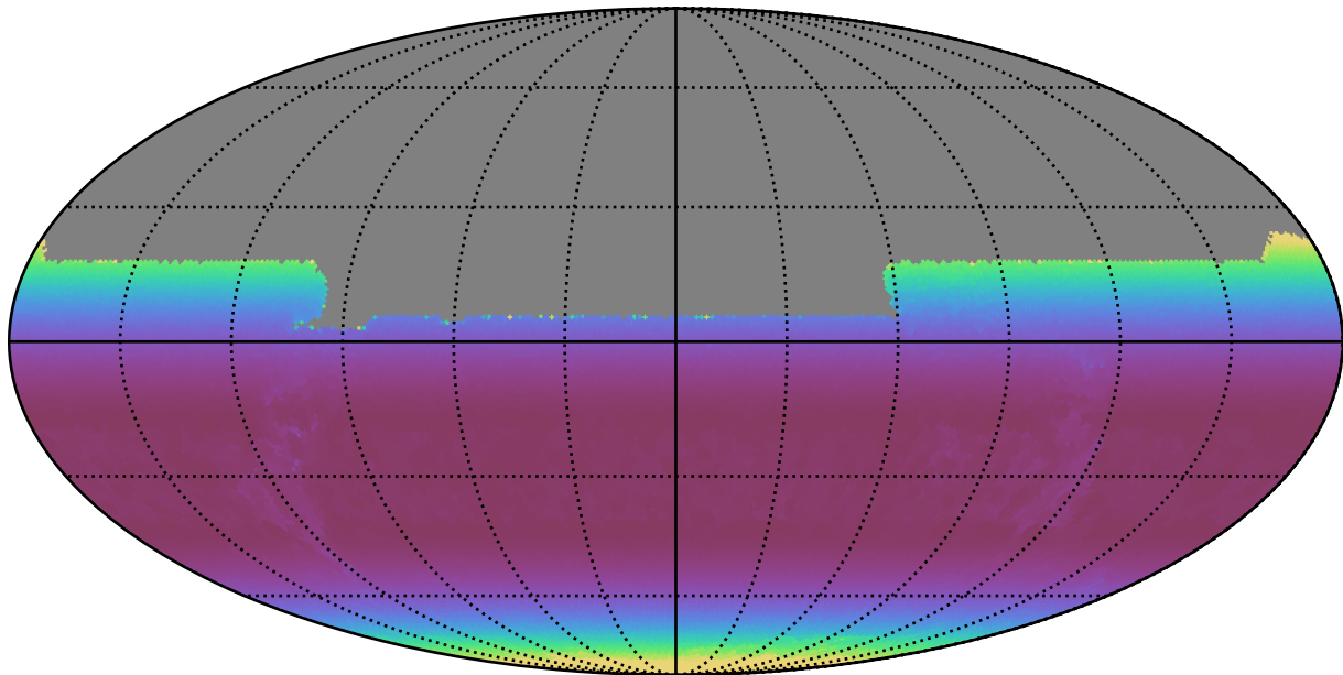
ddf_acor_sf20_lsf0_lsr0_v3.4_10yrs All sky y band: Min airmass
