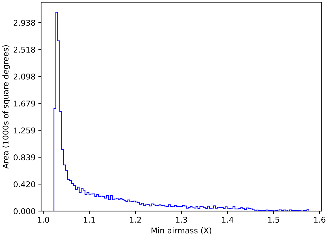
ddf_acor_sf20_lsf0_lsr0_v3.4_10yrs All sky y band: Min airmass
