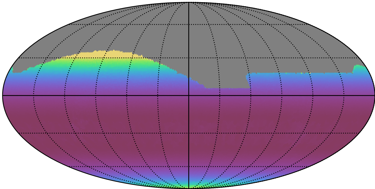
ddf_acor_sf20_lsf0_lsr0_v3.4_10yrs All sky r band: Min airmass
