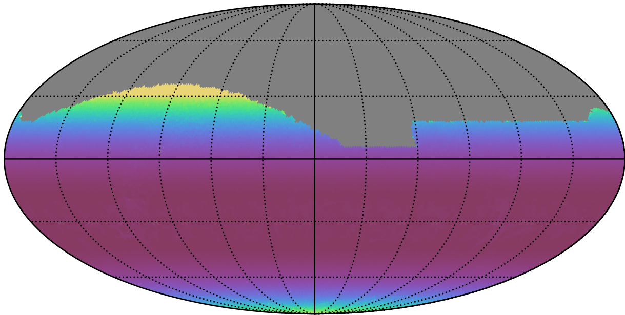
ddf_acor_sf20_lsf0_lsr0_v3.4_10yrs All sky i band: Min airmass
