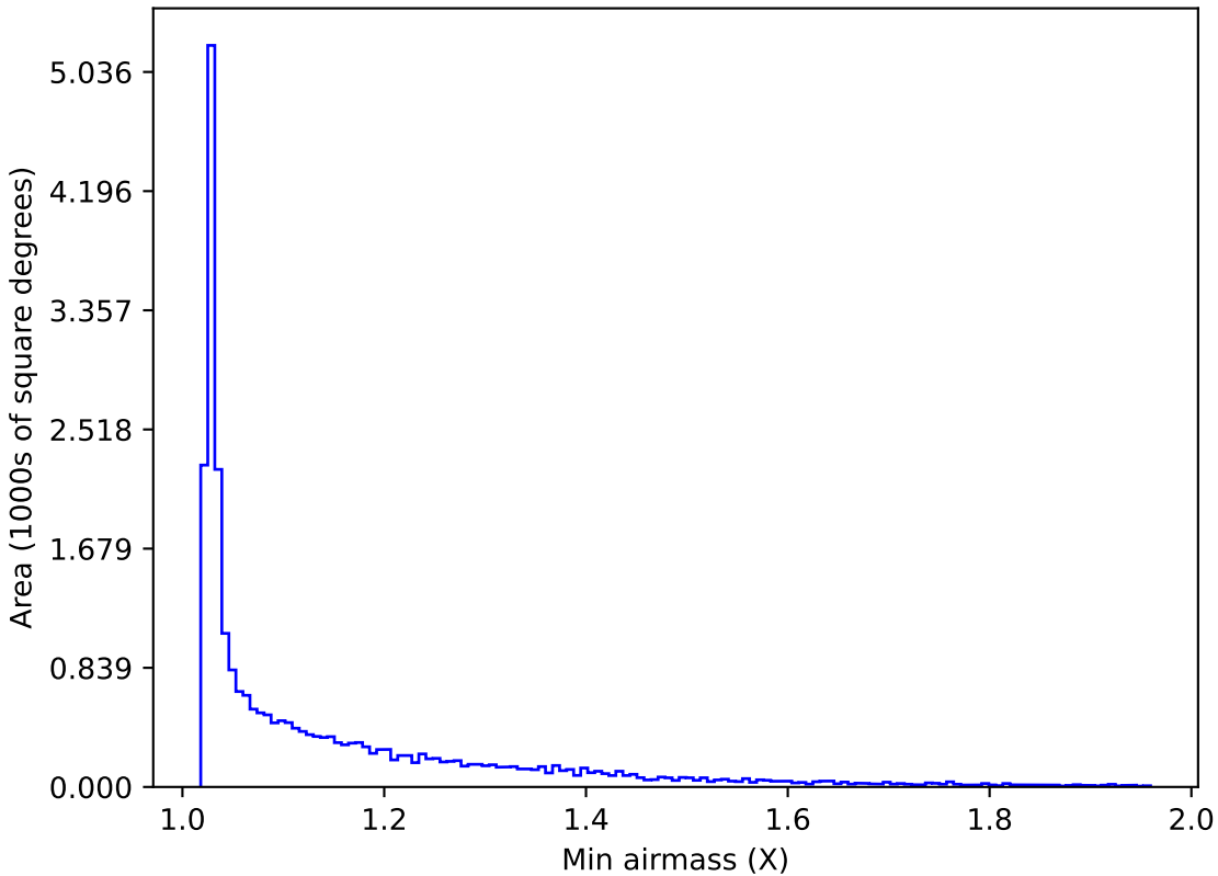
ddf_acor_sf20_lsf0_lsr0_v3.4_10yrs All sky i band: Min airmass
