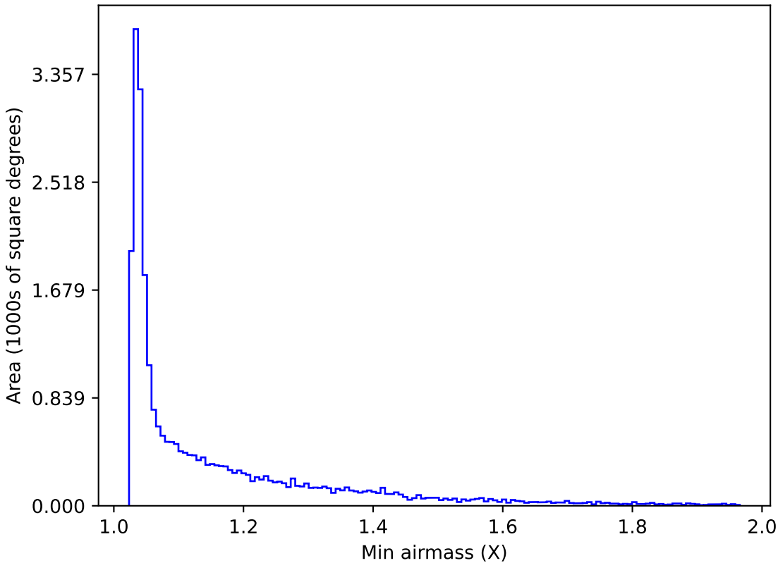
ddf_acor_sf20_lsf0_lsr0_v3.4_10yrs All sky g band: Min airmass
