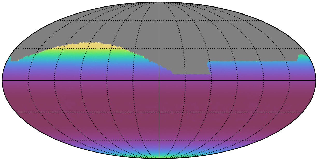
ddf_acor_sf20_lsf0_lsr0_v3.4_10yrs All sky all bands: Min airmass
