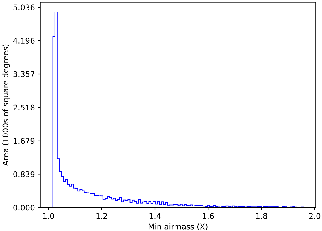
ddf_acor_sf20_lsf0_lsr0_v3.4_10yrs All sky all bands: Min airmass
