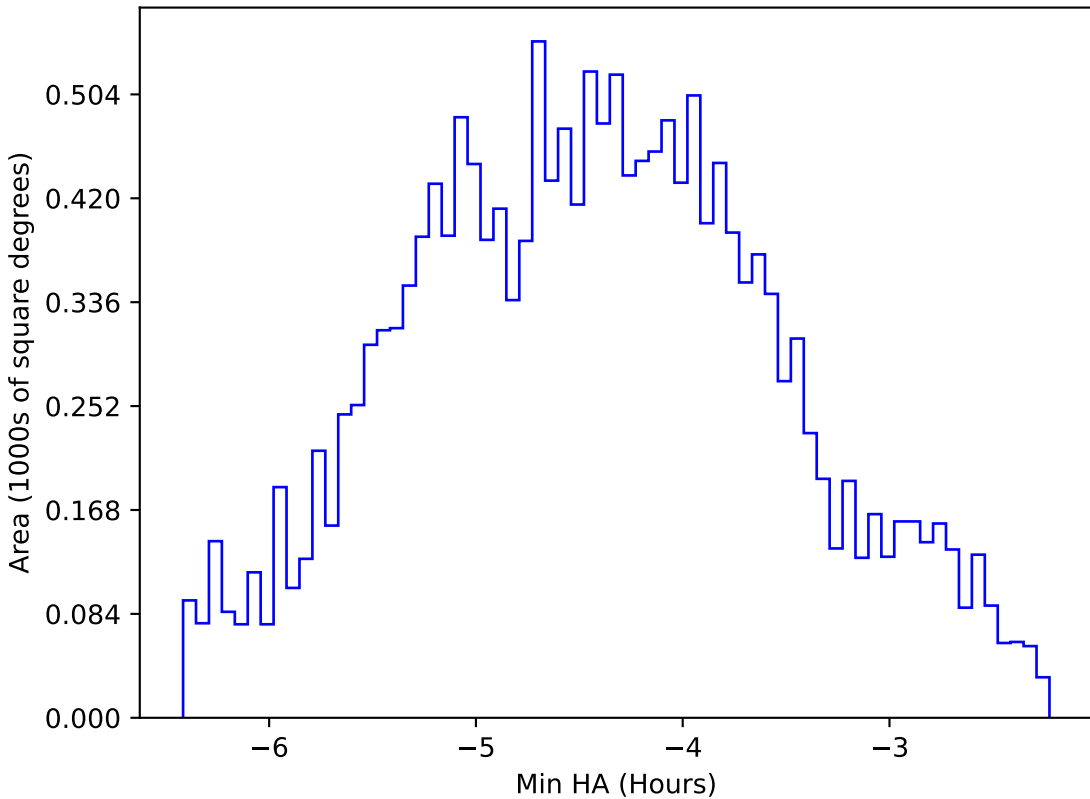
ddf_acor_sf20_ls0_lsr0_v3.4_10yrs WFD z band: Min HA
