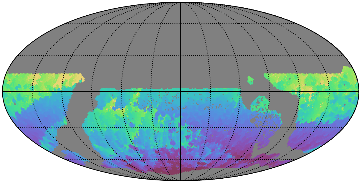
ddf_acor_sf20_lsf0_lsr0_v3.4_10yrs WFD r band: Min HA
