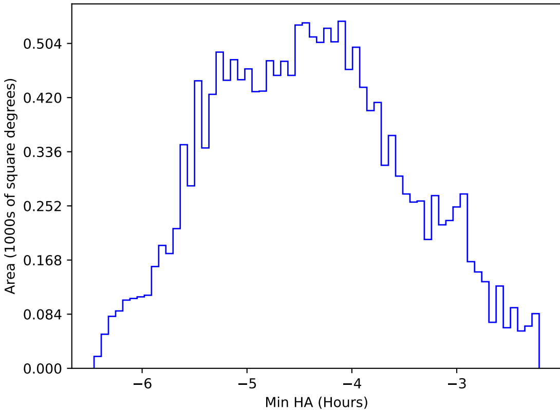
ddf_acor_sf20_lsf0_lsr0_v3.4_10yrs WFD r band: Min HA
