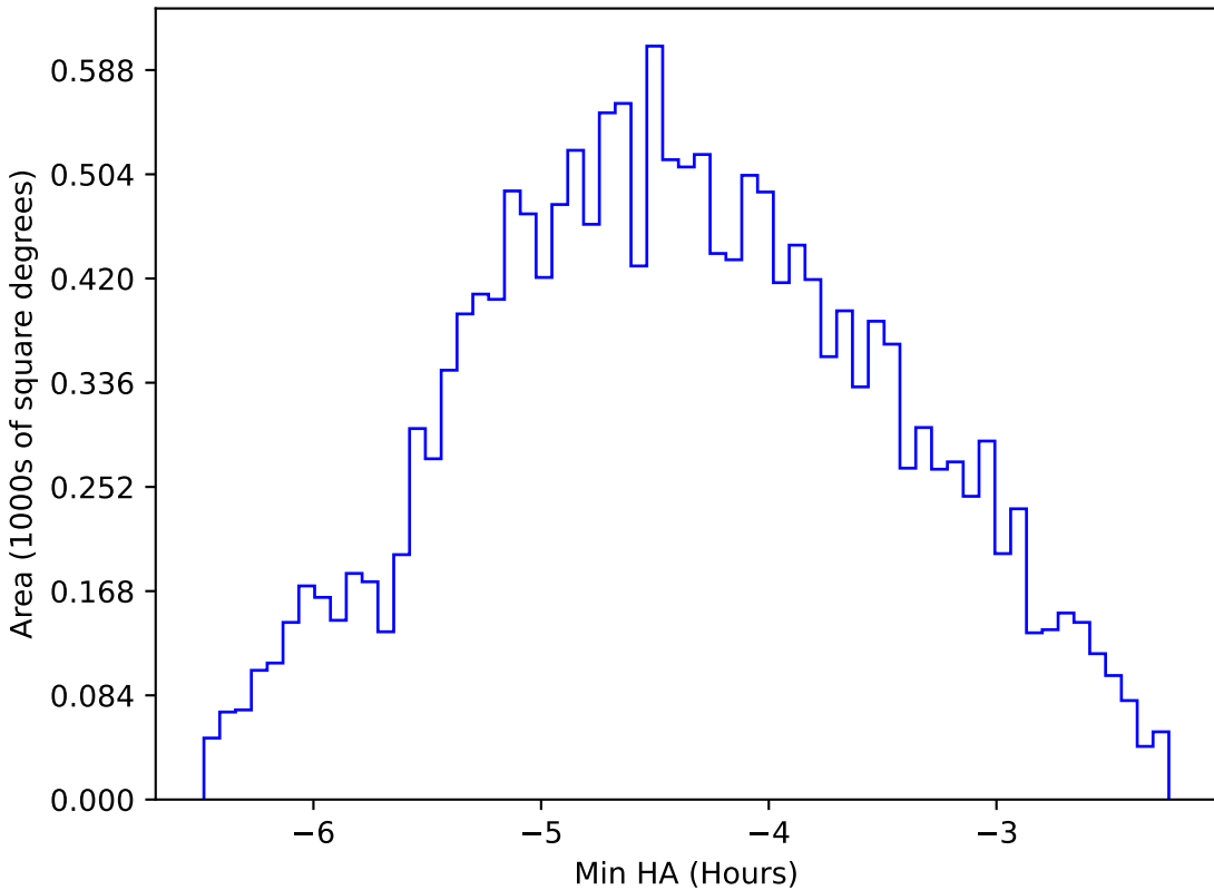
ddf_acor_sf20_lsfo_lsr0_v3.4_10yrs WFD i band: Min HA
