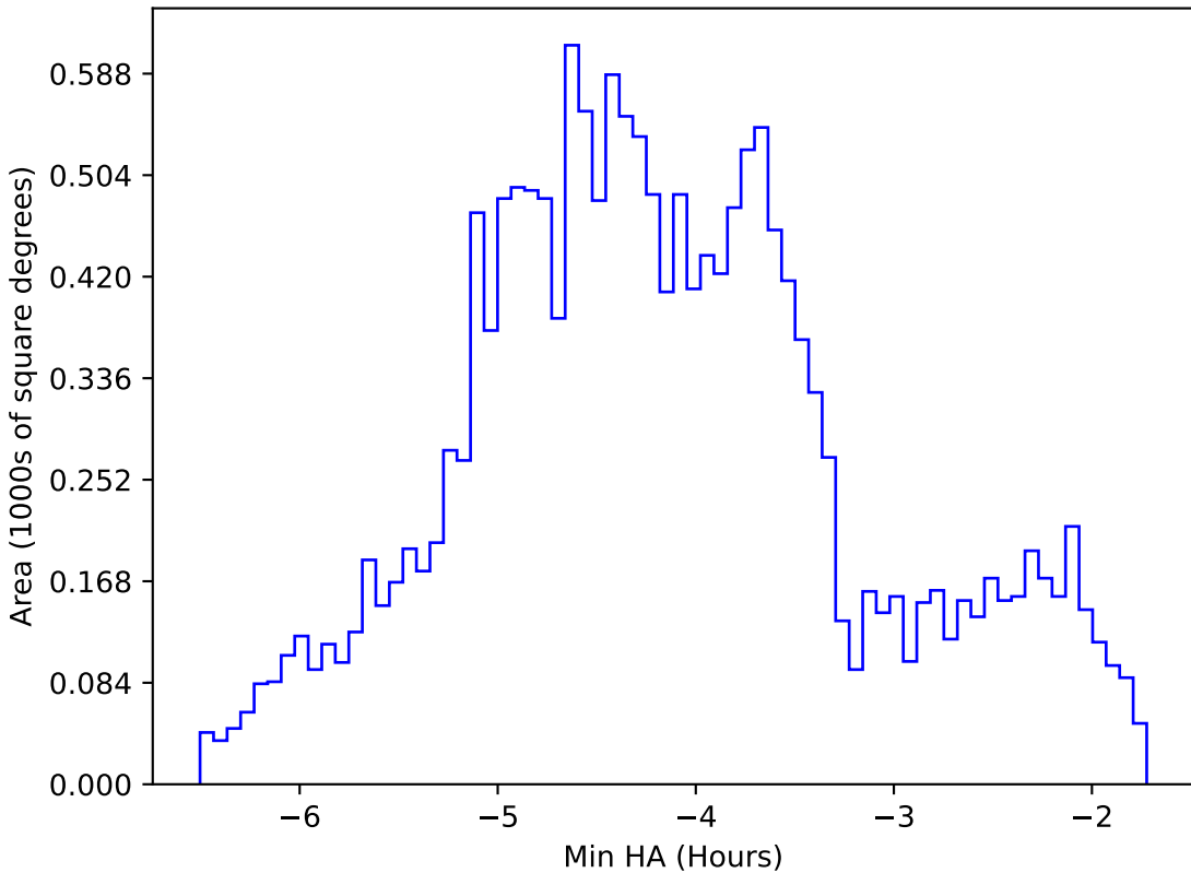
ddf_acor_sf20_lsf0_lsr0_v3.4_10yrs WFD g band: Min HA
