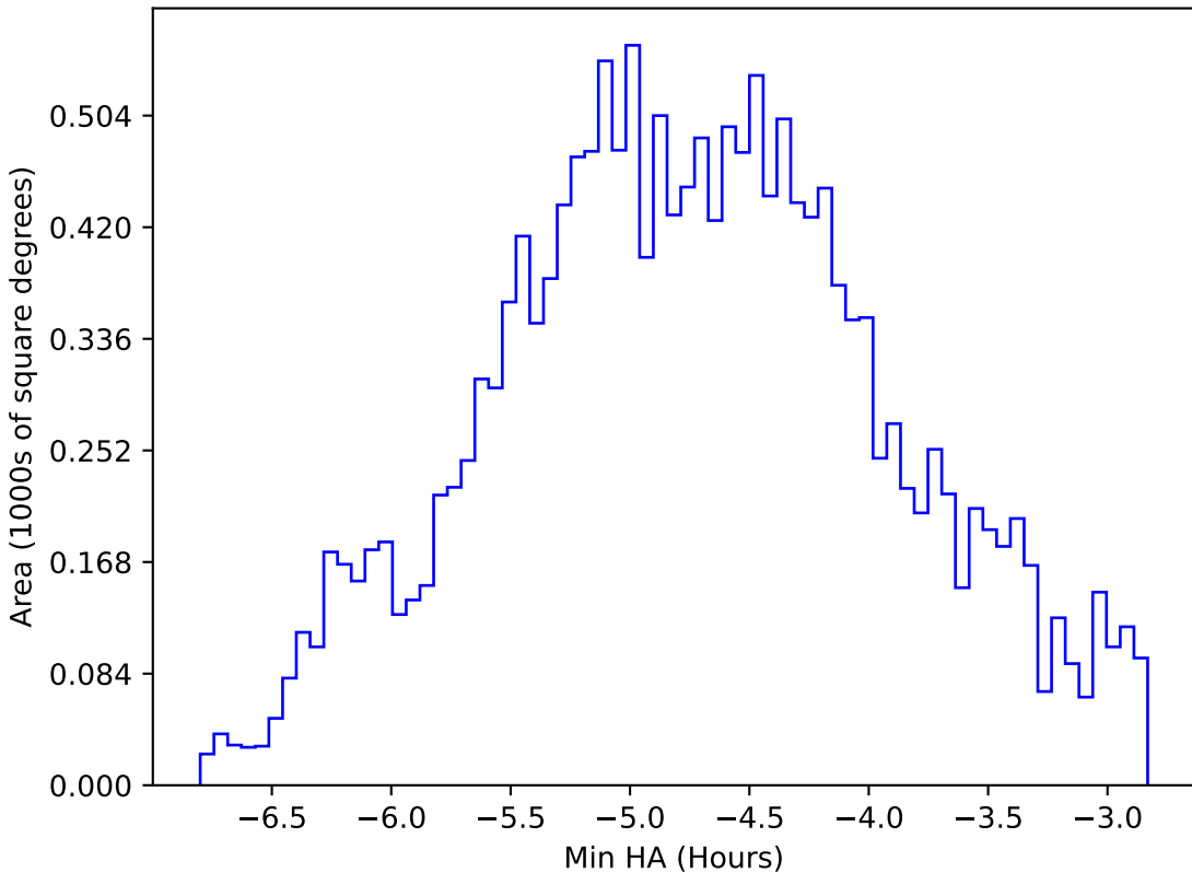
ddf_acor_sf20_lsf0_lsr0_v3.4_10yrs WFD all bands: Min HA
