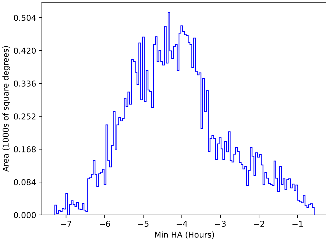
ddf_acor_sf20_lsf0_lsr0_v3.4_10yrs All sky z band: Min HA
