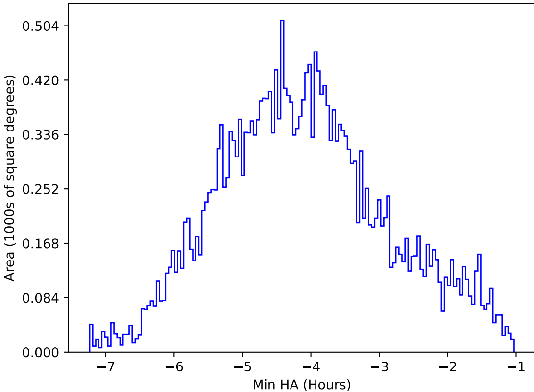
ddf_acor_sf20_lsf0_lsr0_v3.4_10yrs All sky i band: Min HA
