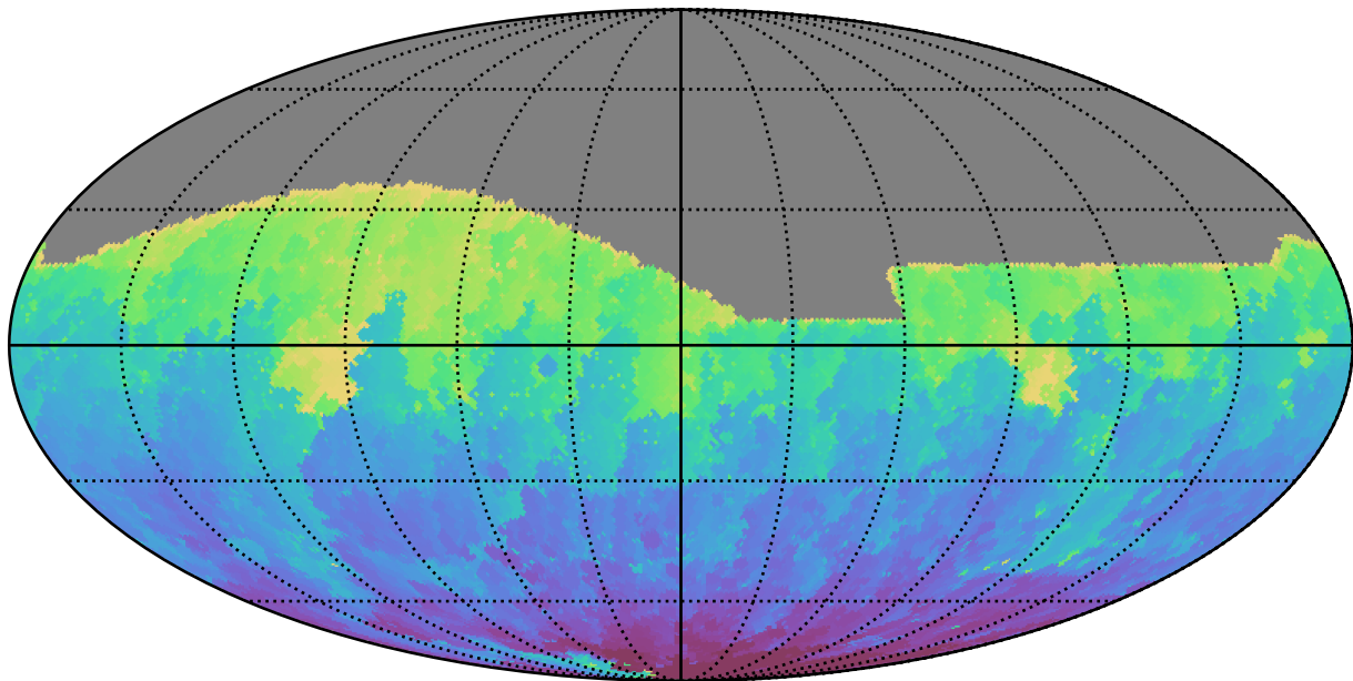
ddf_acor_sf20_lsf0_lsr0_v3.4_10yrs All sky g band: Min HA
