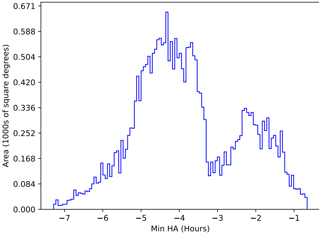
ddf_acor_sf20_lsf0_lsr0_v3.4_10yrs All sky g band: Min HA
