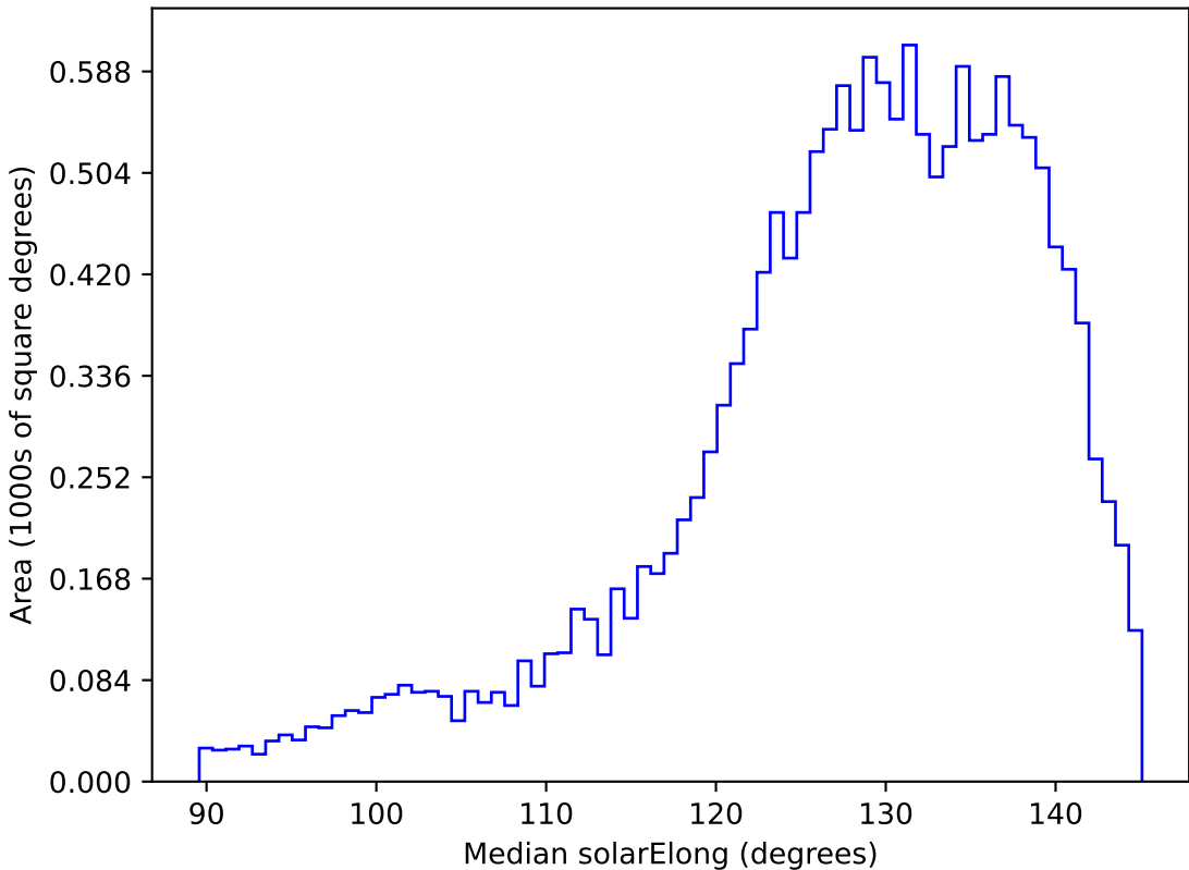
ddf_acor_sf20_lsf0_lsr0_v3.4_10yrs WFD z band: Median solarElong
