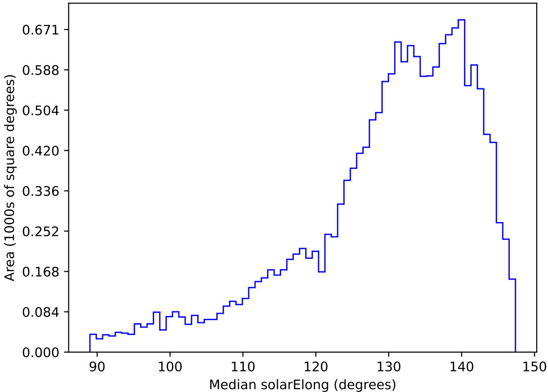
ddf_acor_sf20_ls0_lsr0_v3.4_10yrs WFD y band: Median solarElong
