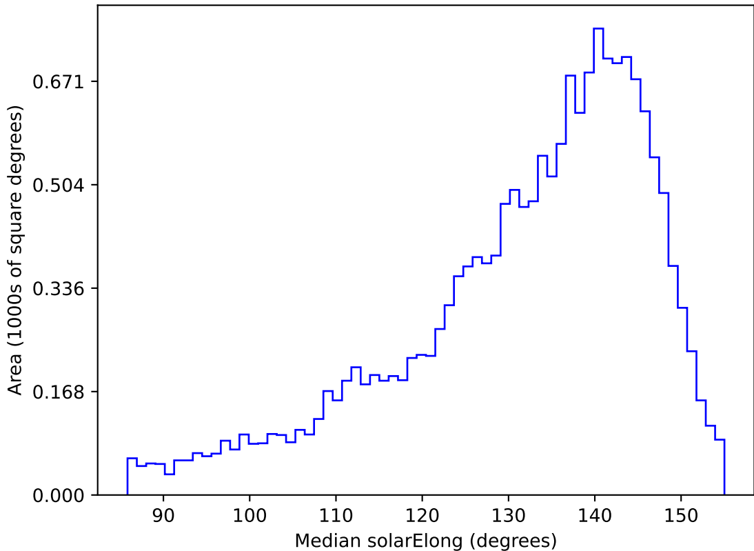
ddf_acor_sf20_ls0_lsr0_v3.4_10yrs WFD u band: Median solarElong
