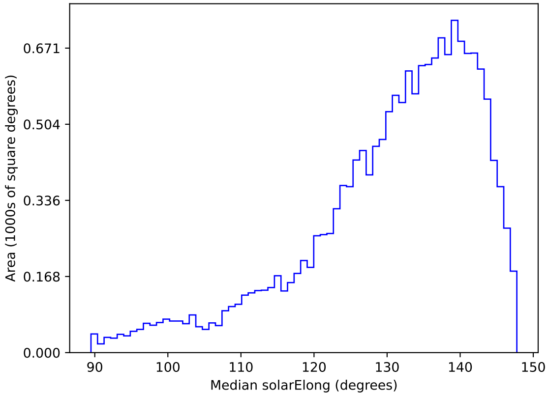
ddf_acor_sf20_lsf0_lsr0_v3.4_10yrs WFD r band: Median solarElong
