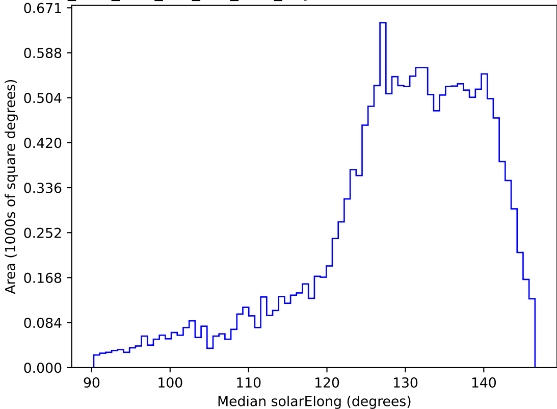
ddf_acor_sf20_lsf0_lsr0_v3.4_10yrs WFD i band: Median solarElong
