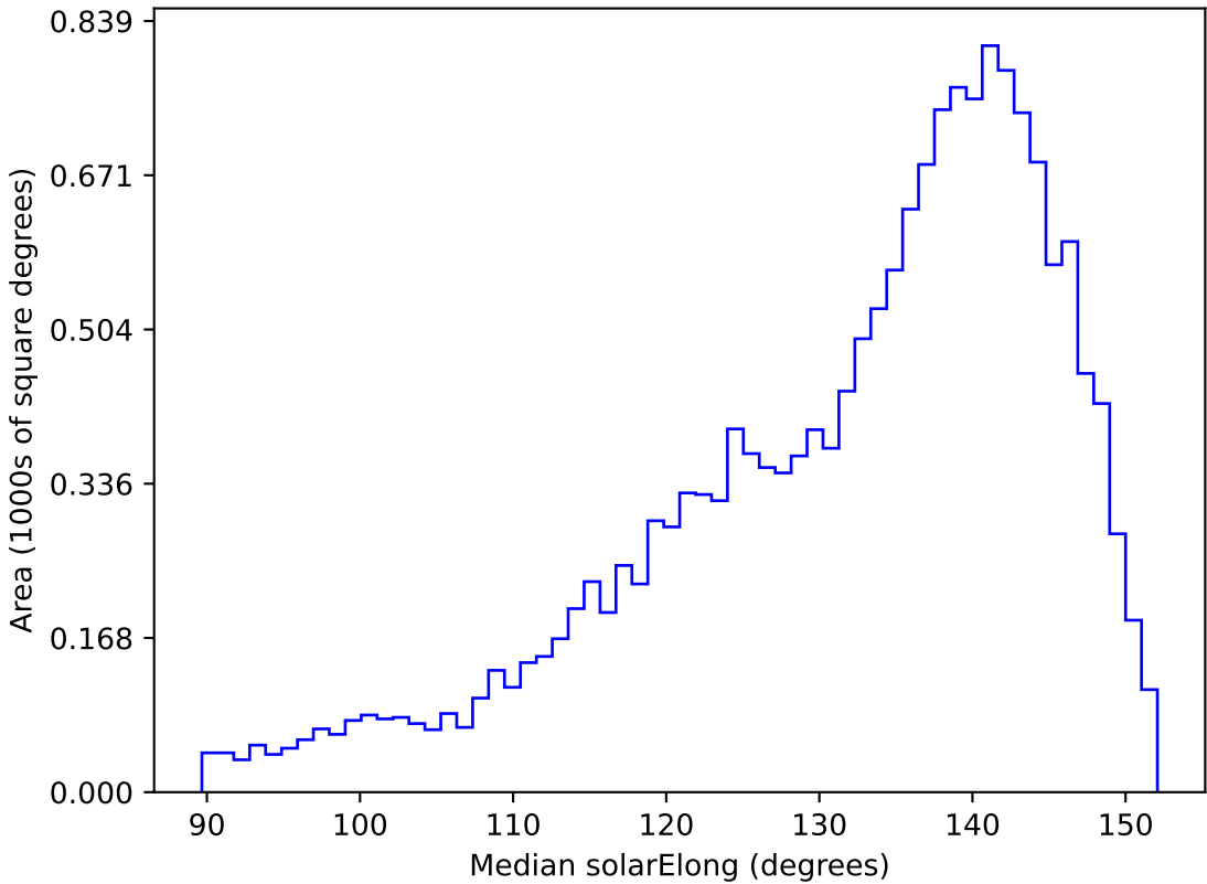
ddf_acor_sf20_lsf0_lsr0_v3.4_10yrs WFD g band: Median solarElong
